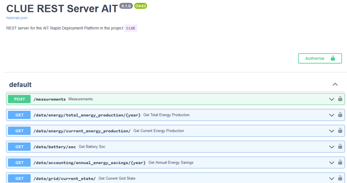
Figure 64: REST endpoints of the AIT RDP
