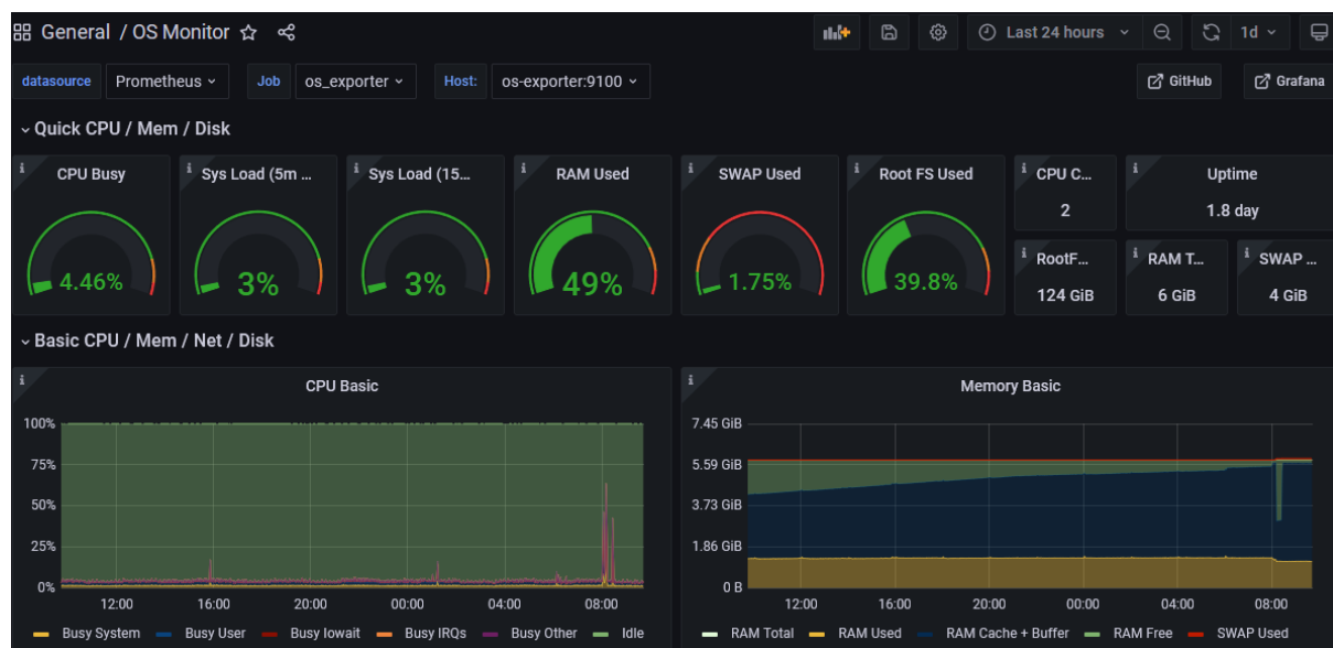
Figure 59: Dashboard of the machine which runs the AIT Rapid Deployment Platform
