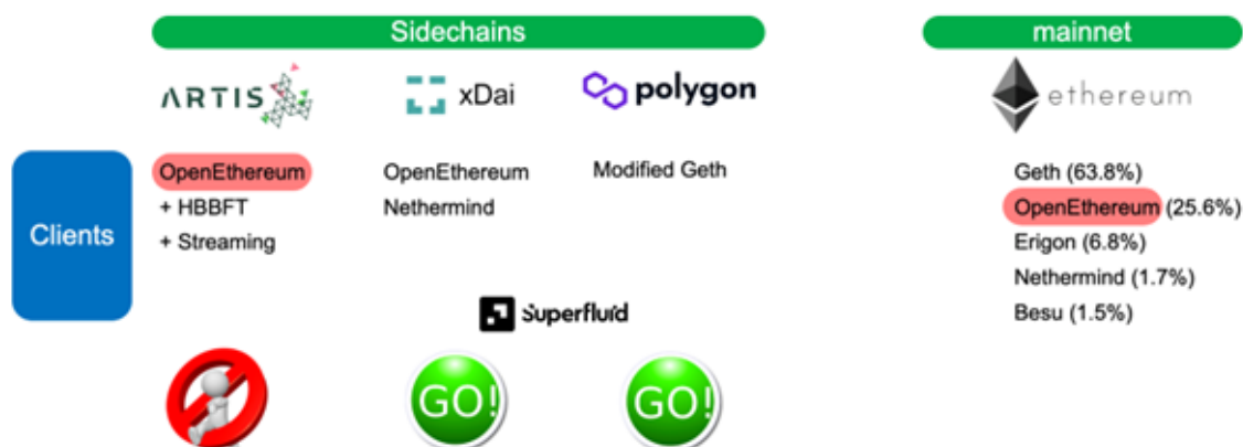
Figure 71: Analysis of programmable blockchains and their suitability for CLUE
