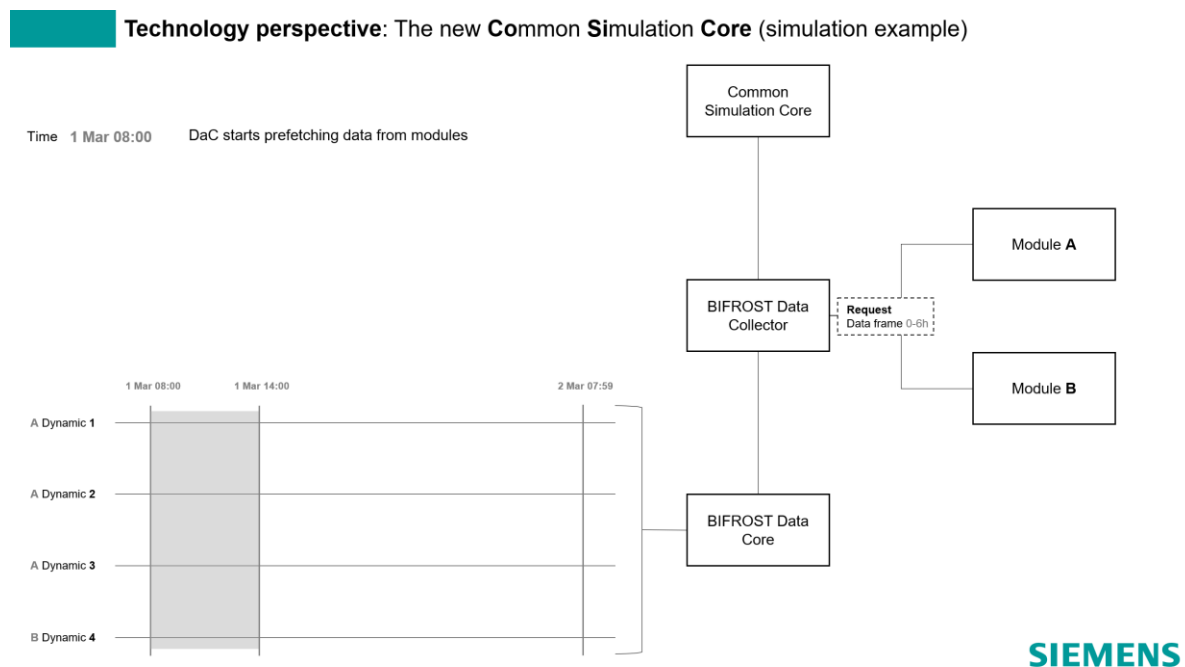
Figure 26: Technology perspective: Prefetch of simulation data
